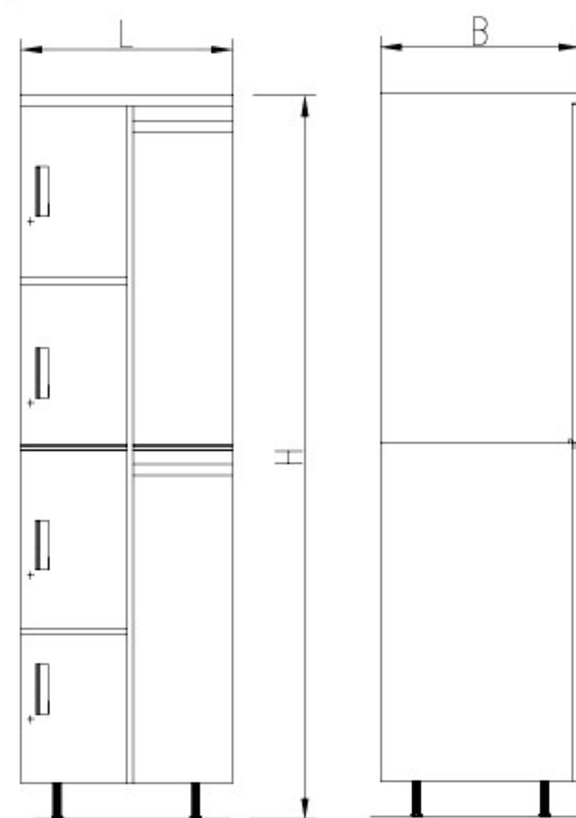
单门衣柜 Single Closet
