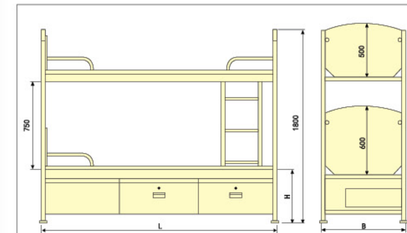
双层柜床 Bunk Bed With Drainers
