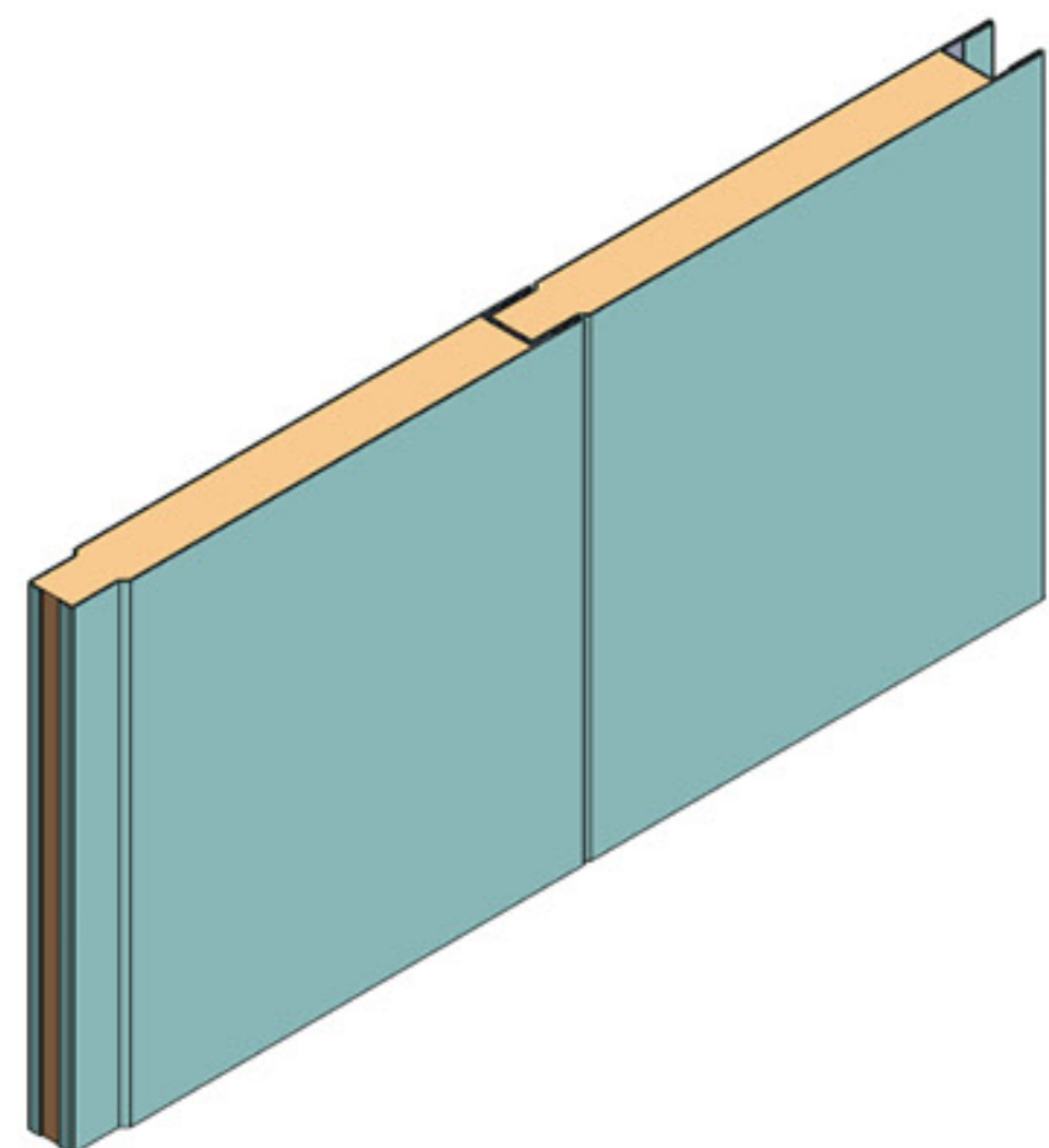
A 型复合岩棉天花板 Type A Composite Rock Wool Ceilings
